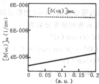
Fig. 4 The minimum detectable absorbance \delta(\omega_1)_{sig} as the function of the total loss \sigma , for \eta = 0.9 , S_{dp} = 0.15 , M = 0.1 ; l = 10 cm, \langle I_1 \rangle = 1 mW, B = 30 kHz
