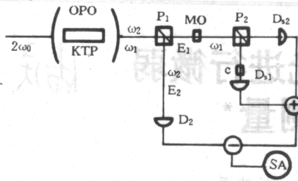
Fig. 1 Scheme for absorption spectroscopy measurement with twin beams
